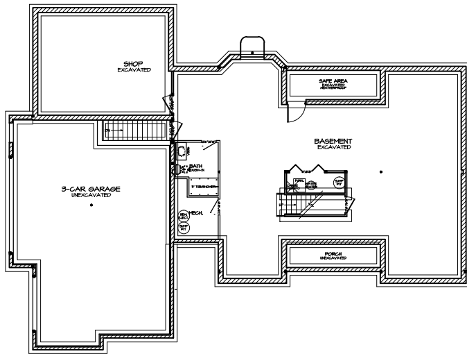
FOUNDATION PLAN A-1
