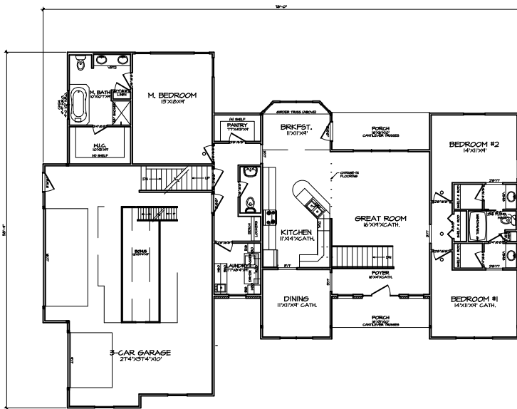
FIRST FLOOR PLAN A-1
